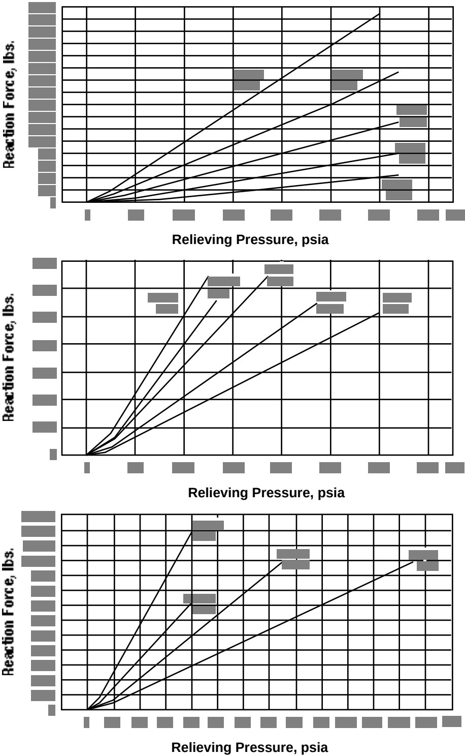
Figure F7-9 Steam
