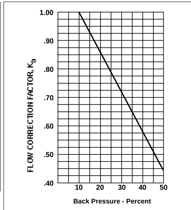
Figure F7-2B Series BP Valves - 10% Overpressure
